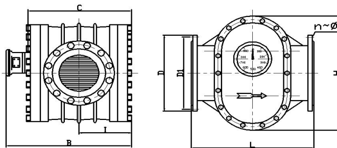
DN50 (heavy type)~DN100
